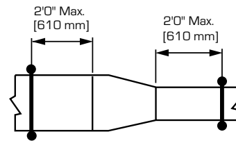
Figure 6-5 STRAIGHT REDUCER
