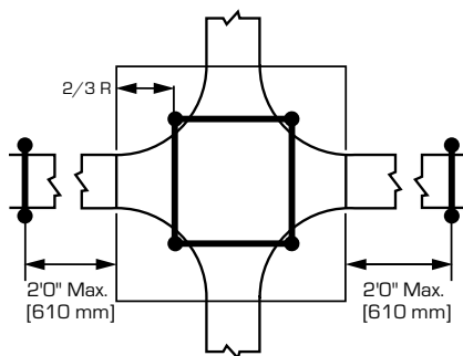
Figure 6-3 HORIZONTAL CROSS
