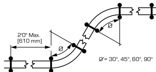
Figure 6-7 VERTICAL ELBOWS
