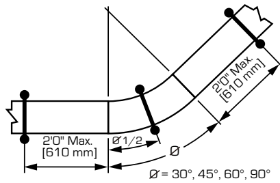
Figure 6-1 HORIZONTAL ELBOWS
