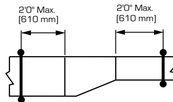
Figure 6-6 OFFSET REDUCER
