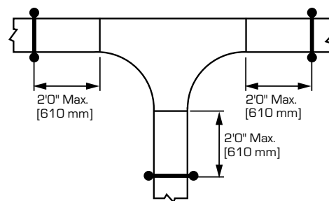
Figure 6-8 VERTICAL TEE
