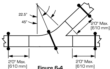
Figure 6-4 HORIZONTAL WYE
