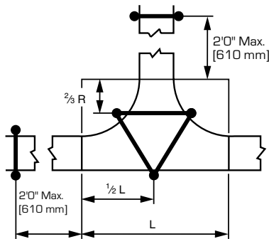
Figure 6-2 HORIZONTAL TEE
